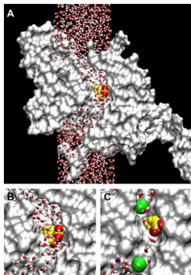
FIGURE 1 (A) The MD system with the CIC-0 monomer cross sectioned along the pore and represented by a solvent accessible surface. The water column extends to 90 Å total height. Glu-148 is highlighted at the center of the pore, with the two negatively charged oxygens of its side chain in red. (B) Detail view of the central region. (C) The same region in a model with a smaller minimum pore diameter ( \approx 4 Å). Two \text{Cl}^- ions are shown in green, radius 1.81 Å.
