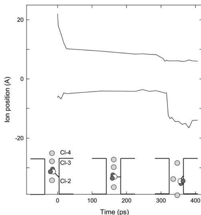
FIGURE 4 Fast gate opening to allow inward conduction. The upper curve shows the z position of \text{Cl} -4, and the lower curve shows the distance between this ion and \text{Cl} -3. \text{Cl} -4 is constrained near specified positions during the simulation, while the other ions and the Glu-148 side chain are free. Initial positions of ions and the side chain are sketched in the first inset. When \text{Cl} -4 is brought into the pore, the resulting configuration ( middle inset ) is relatively stable for \sim 300 ps. But the side chain eventually retreats against the wall of the pore for a moment and \text{Cl} -3 slips past ( right-hand inset ).
